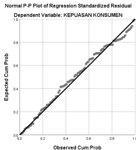
Gambar 4.1.1 Hasil Uji Normalitas (P-P Plot of Regression)
