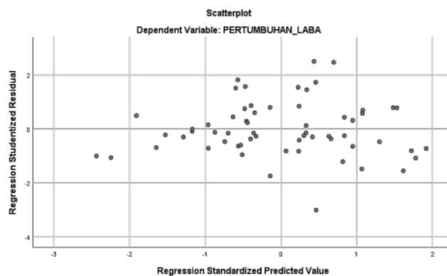
Gambar 3. Scatterplot
