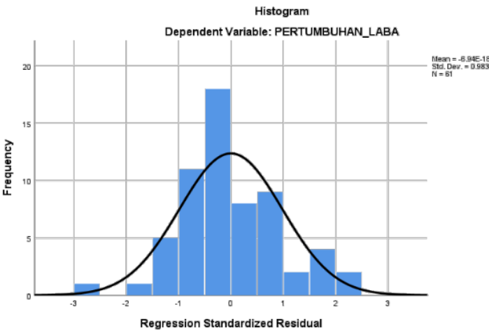
Gambar 1. Histogram
