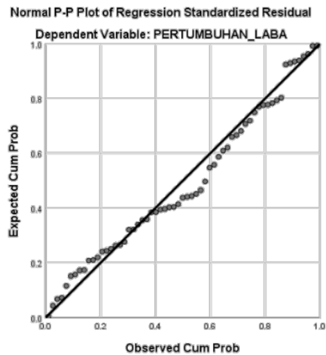
Gambar 2. P-P Plot
