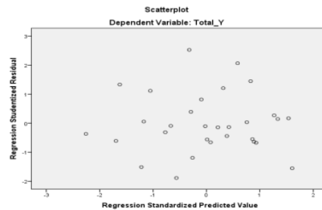
Gambar Scaterplot
